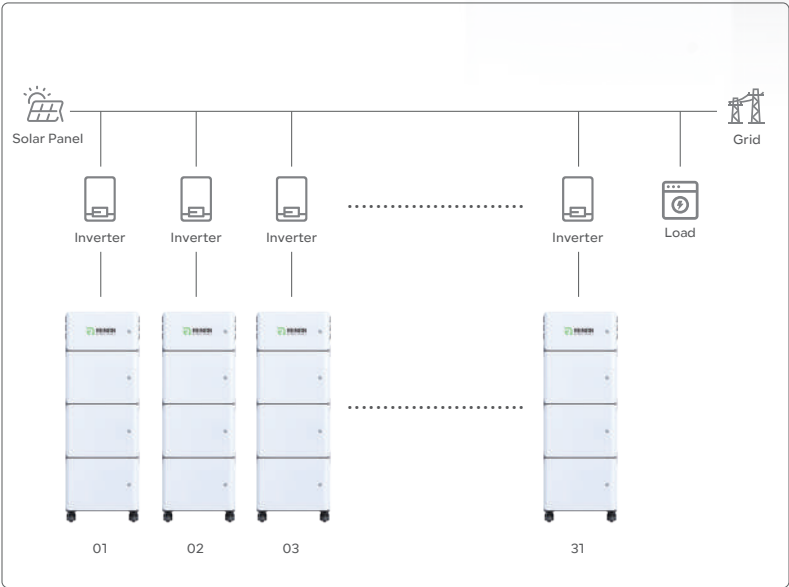
System Layout
